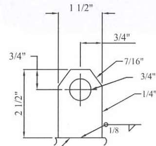
DETAIL H LIFTING LUG
