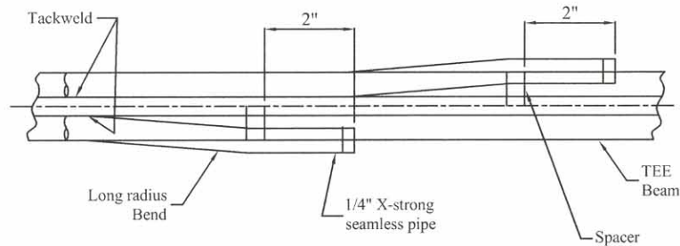
SECTION G-G
