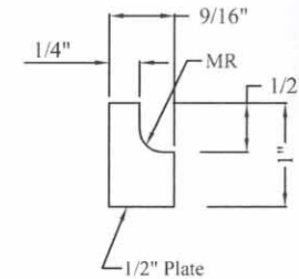
DETAIL E SPACER
